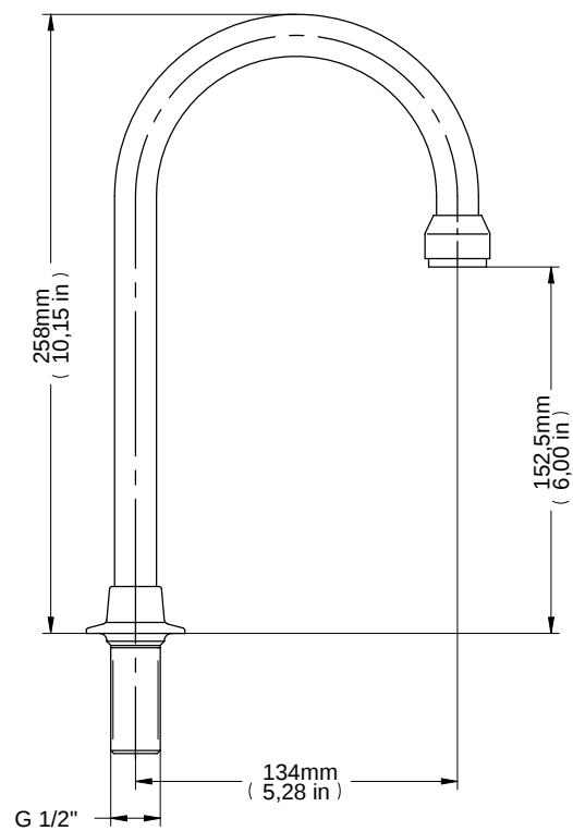
BICA LAVATORIO MESA HOSPITALAR P/ VALVULAS DE PISO PEMATIC DECK-MOUNT SPOUT FOR HOSPITALS/CLINICS PICO HOSPITALARIO MESA
